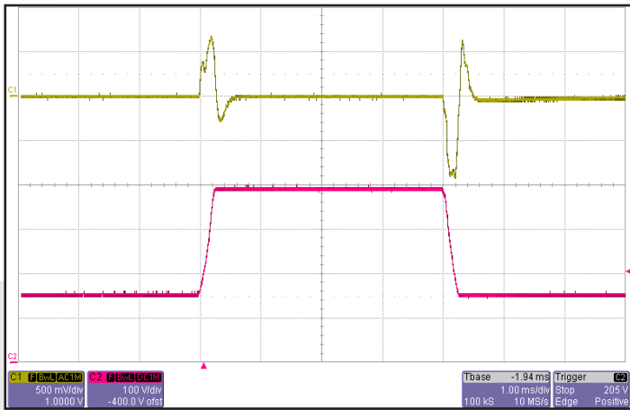
Figure 13: Output voltage response to step-change in input voltage (155V - 400V - 155V) in 250 \mu S. Load cap: 10 \mu F, 100m \Omega ESR tantalum cap and 1 \mu F ceramic cap. Ch 1: Vout (500mV/div). Ch 2: Vin (100V/div).
